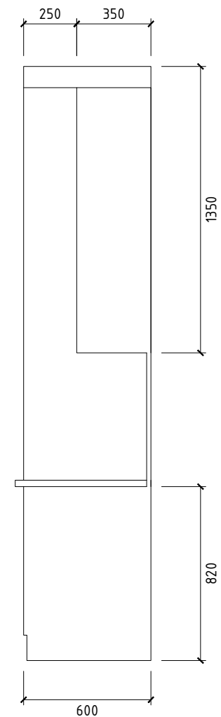
KP - KABINET PANTRY TAMPAK SAMPIING SKALA 1 : 25
