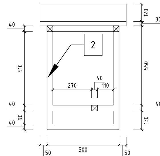
MP - MEJA PRIVATE BOOTH POTONGAN SKALA 1 : 15
