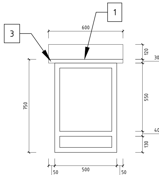
MP - MEJA PRIVATE BOOTH TAMPAK SAMPIING SKALA 1 : 15
