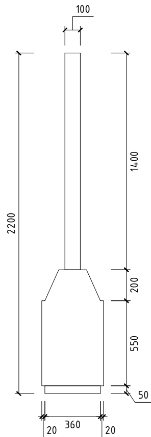
PB - PLANTER BOX TAMPAK SAMPIING SKALA 1 : 25
