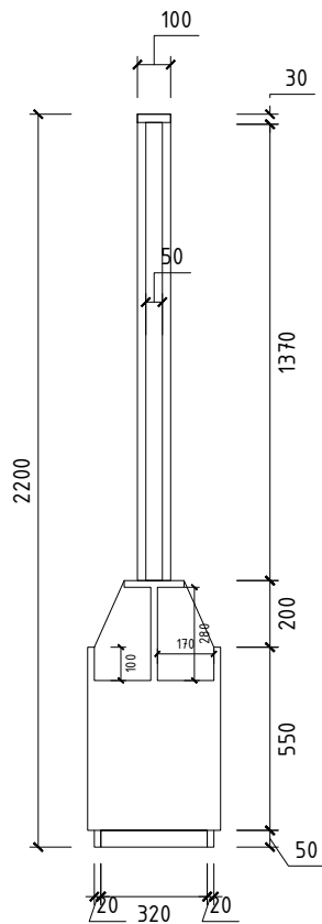
PB - PLANTER BOX POTONGAN SKALA 1 : 25
